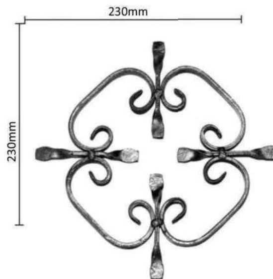
WR701/P - 12mm x 5mm WR701/HM- 12mm x 5mm Dim - 230mm x 230mm
