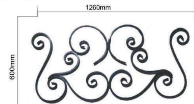
WGP0030 12mm Square Bar 25mm x 5mm Flat Bar Dim - 1260mm x 600mm
