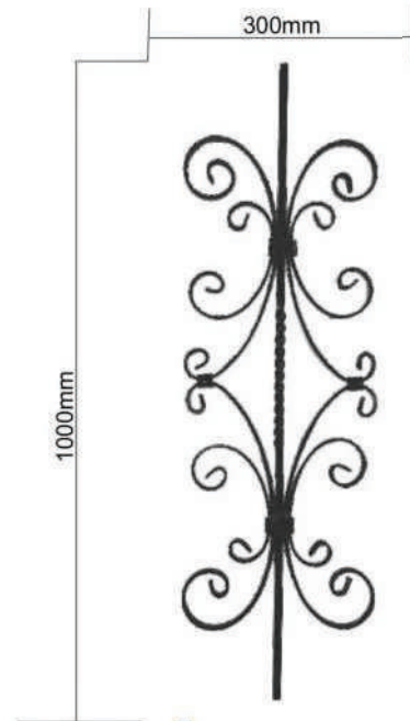
WUP 513 12mm Square Bar/12mm x 5mm Flat Bar Dim 300mm x 1000mm
