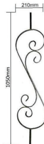
WP26/268/P - 12mm x 12mm/12mm x 5mm WP26/268/HM - 12mm x 12mm/12mm x 5mm Dim - 210mm x 1050mm
