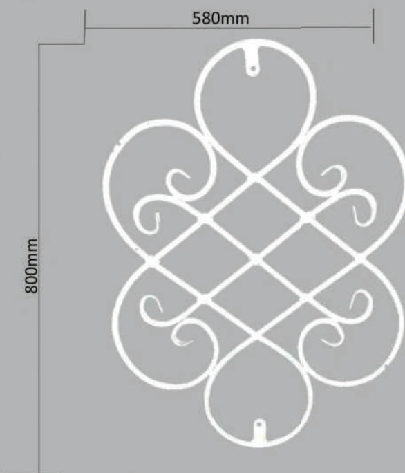
WPU0005 Wall Panel 12mm Round Bar Dim 580mm x 800mm
