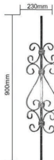
WP26/293/P - 12mm x 12mm/12mm x 5mm WP26/293/HM - 12mm x 12mm/12mm x 5mm WP26/293/TW - 12mm x 12mm/12mm x 5mm Dim - 230mm x 900mm
