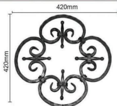
WR505/P - 12mm x 12mm WR505/HM- 12mm x 12mm Dim - 420mm x 420mm
