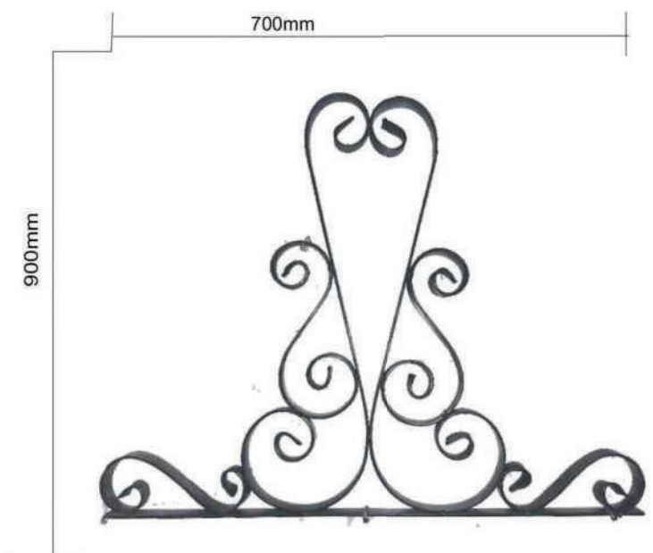
WGP0029 40mm x 5mm Flat Bar Dim - 700mm x 900mm
