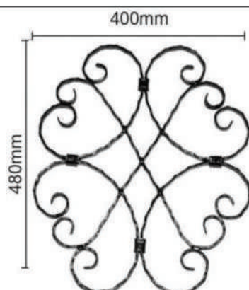
WGYD5517/P - 12mm x 12mm WGYD5517/HM - 12mm x 12mm Dim - 400mm x 480mm
