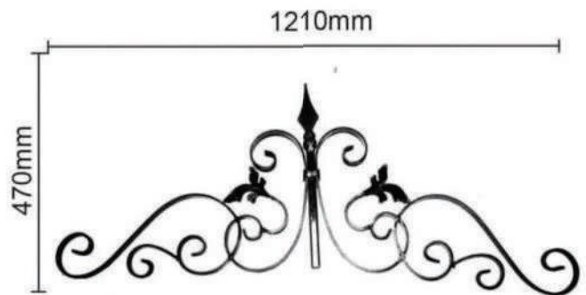
WTOP106/P - 20mm x 5mm/20mm x 20mm/1.6mm Tube Dim - 1210mm x 470mm
