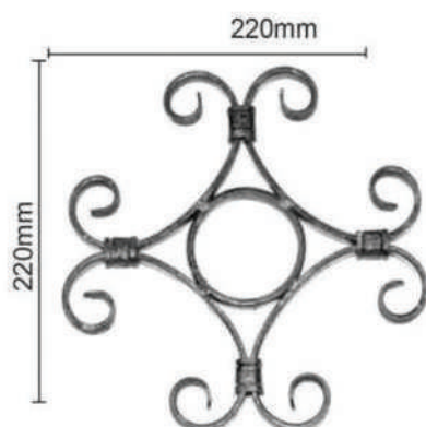
WR1001/P - 12mm x 5mm WR1001/HM- 12mm x 5mm Dim - 220mm x 220mm
