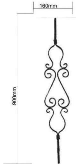
WUP 14662 12mm Square Bar/12mm x 5mm Flat Bar Dim 160mm x 900mm
