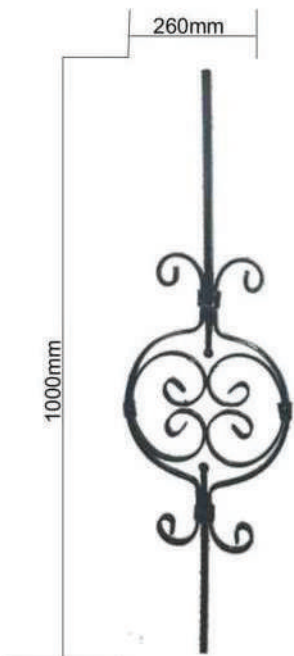
WUP5116 12mm Square Bar/12.5mm Flat Bar Dim 260mm x 1000mm
