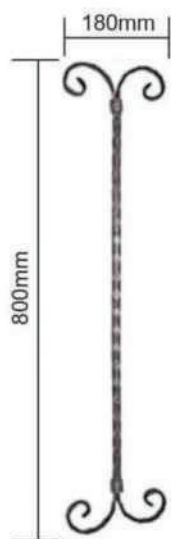
WP7205/P - 12mm x 12mm / 12mm x 5mm WP7205/HM - 12mm x 12mm / 12mm x 5mm Dim - 180mm x 800mm
