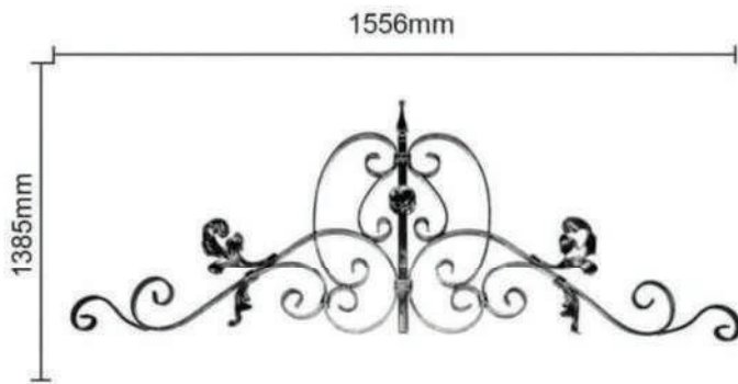
WTOP206/P - 20mm x 5mm/20mm x 20mm/1.6mm Tube Dim - 1556mm x 1385mm
