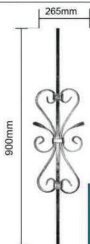
WP26/298/P - 12mm x 12mm/12mm x 5mm WP26/298/HM - 12mm x 12mm/12mm x 5mm WP26/298/TW - 12mm x 12mm/12mm x 5mm Dim - 265mm x 900mm
