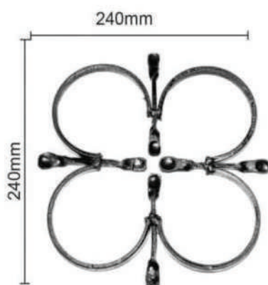
WR601/P - 12mm x 5mm WR601/HM- 12mm x 5mm Dim - 240mm x 240mm
