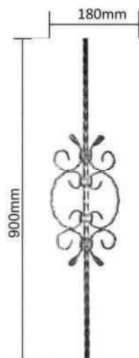
WP26/273/P - 12mm x 12mm/12mm x 5mm WP26/273/HM - 12mm x 12mm/12mm x 5mm WP26/273/TW - 12mm x 12mm/12mm x 5mm Dim - 180mm x 900mm
