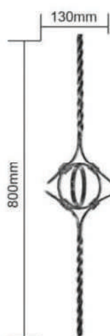
WP4701/D/P - 12mm x 5mm/12mm x 12mm WP4701/D/HM - 12mm x 5mm/12mm x 12mm WP4701/D/TW - 12mm x 5mm/12mm x 12mm Dim - 130mm x 800mm
