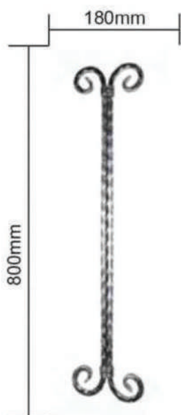
WP011/P - 12mm X 12mm WP011/HM - 12mm X 12mm Dim - 180mm x 800mm
