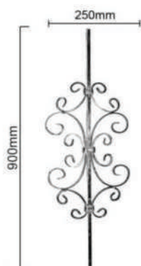
WP26/308/P - 12mm x 12mm/12mm x 5mm WP26/308/HM - 12mm x 12mm/12mm x 5mm Dim - 250mm x 900mm
