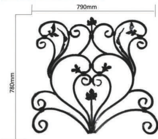
WGP 0025 12mm Square Bar Dim 790mm x 780mm
