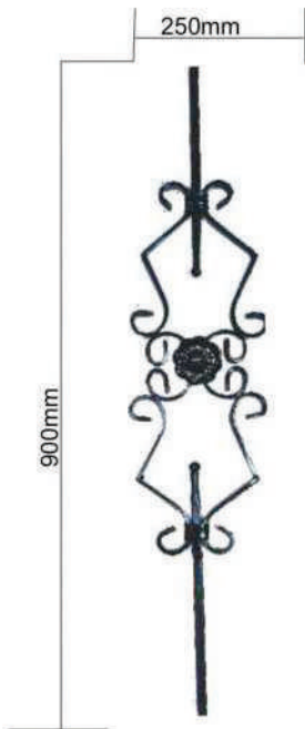
WUP 14661 12mm Square Bar/12.5mm Flat Bar Dim 250mm x 900mm
