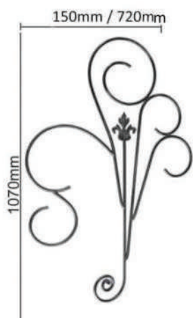
WHM1426/A/L - 12mm Round Bar WHM1426/A/R - 12mm Round Bar Dim - 150mm / 720mm x 1070mm
