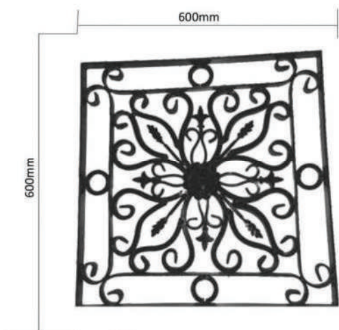
WGP 0022 12mm Square Bar 12x5mm Flat Bar Dim 600mm x 600mm
