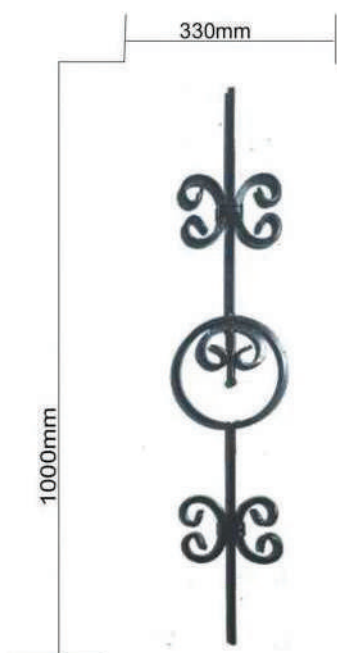
WUP2704 12mm Square Bar Dim 330mm x 1000mm
