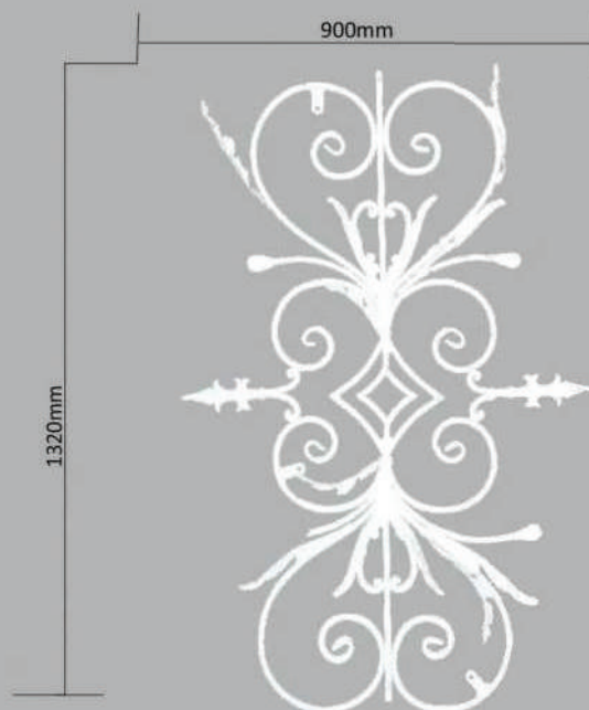
WPU0007 Wall Panel 12mm Square Bar and 12mm Round Bar Dim 900mm x 1320mm
