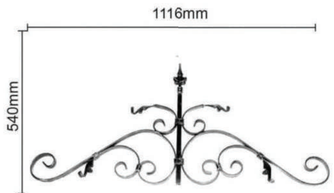
WTOP306/P - 20mm x 5mm/20mm x 20mm/1.6mm Tube Dim - 1116mm x 540mm
