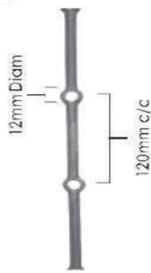
PR112 RD Pierced bar 2m (length)
