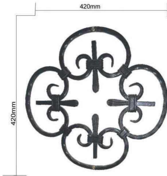
WRN0001 12mm Square Bar Dim - 420mm x 420mm
