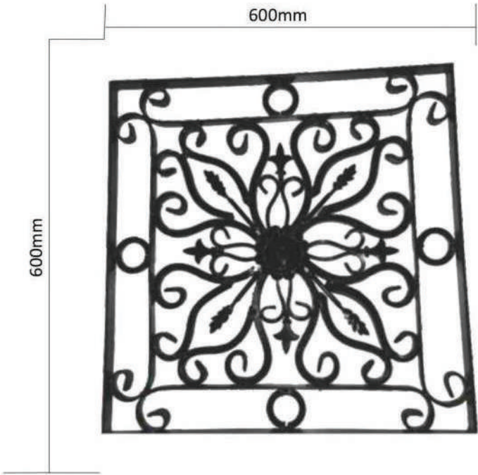
WGP 0022 12mm Square Bar 12x5mm Flat Bar Dim 600mm x 600mm
