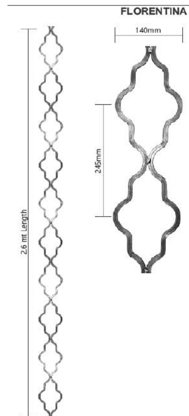
PR-113 Florentine Bar 12 x 12 x 2.6M
