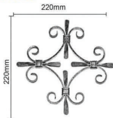
WR1101/P - 12mm x 5mm WR1101/HM - 12mm x 5mm Dim - 220mm x 220mm
