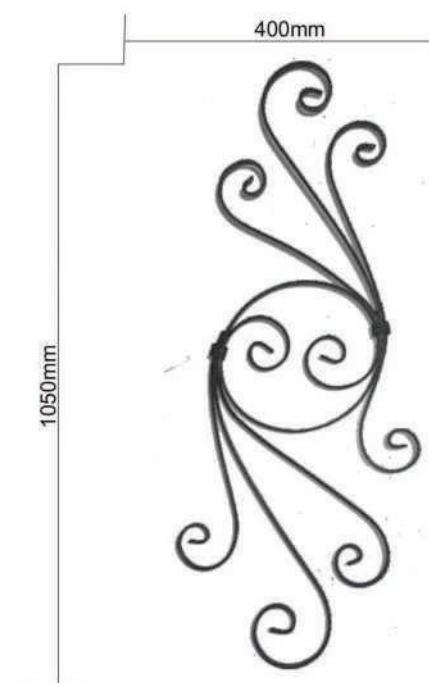
WPU0028 12mm x 5mm Flat Bar Dim - 400mm x 1050mm
